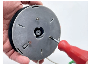
Tighten the three internal screws
